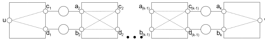
Fig. 2: General Square Graph Decomposition
