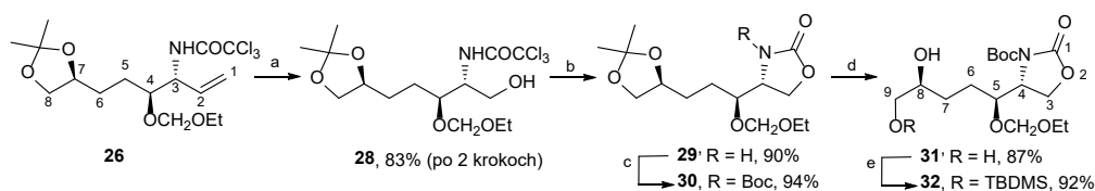
Schéma 2. Činidlá a podmienky: (a) (i) \text{O}_3 , MeOH, -78 °C, 30 min; (ii) \text{NaBH}_4 , MeOH, -78 °C → 0 °C, 1 h; (b) (i) DBU, \text{CH}_2\text{Cl}_2 , rt, 4 h; (c) \text{Boc}_2\text{O} , \text{Et}_3\text{N} , DMAP, \text{CH}_2\text{Cl}_2 , 0 °C → rt, 15 min; (d) p -TsOH, MeOH, 50 °C, 30 min; (e) (i) TBDMSCl, imidazol, \text{CH}_2\text{Cl}_2 , rt, 1 h.
