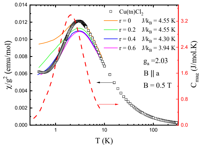
Fig. 3 Temperature dependence of reduced susceptibility \chi normalized by the g -factor, showing collapse onto a universal curve at high temperatures. Solid lines represent Monte Carlo simulation for S=1/2 HAF of a rectangular lattice [3,6]. The dashed line corresponds to the experimental specific heat results in B = 0 T [3].
