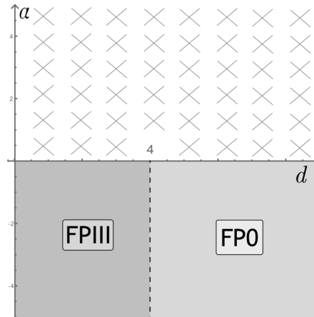
Fig. 2: Phase diagram of IR stability regimes of fixed points in the plane (d, \alpha)
