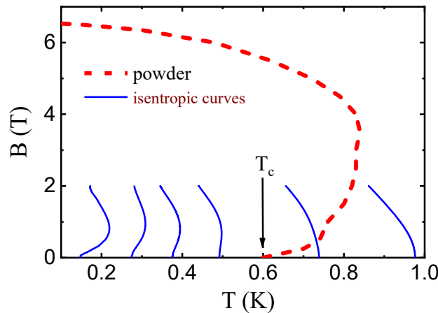
Fig. 6 Magnetic phase diagram of Cu(tn)Cl 2 of powder sample [1] and isentropic (adiabatic magnetizing) curves [9].
