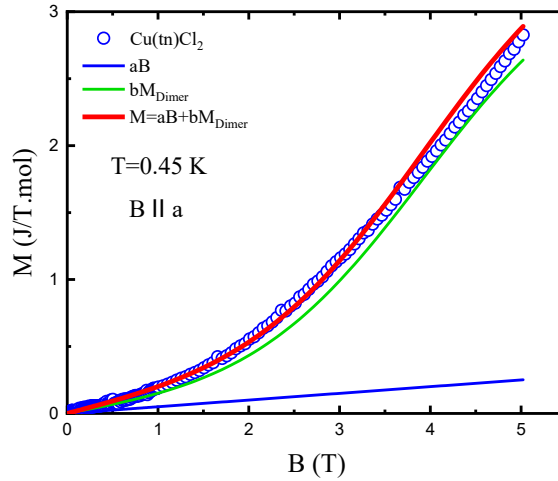
Fig. 5 Field dependence of magnetization of Cu(tn)Cl 2 single crystal. The experimental results (blue circles), the contribution of the rectangular lattice (blue line), the contribution of the dimer model (green line), and the total magnetization calculated from eq. 1 (red line).
