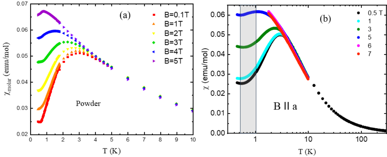
Fig. 2 Temperature dependence of magnetic susceptibility for (a) powder sample in magnetic fields ranging from B = 0.1 up to 5 T. (b) Single crystal sample measured in constant magnetic fields applied parallel to the crystallographic a -axis with values from B = 0.5 up to 7 T. The shaded area refers to the phase transition region reported in [3].
