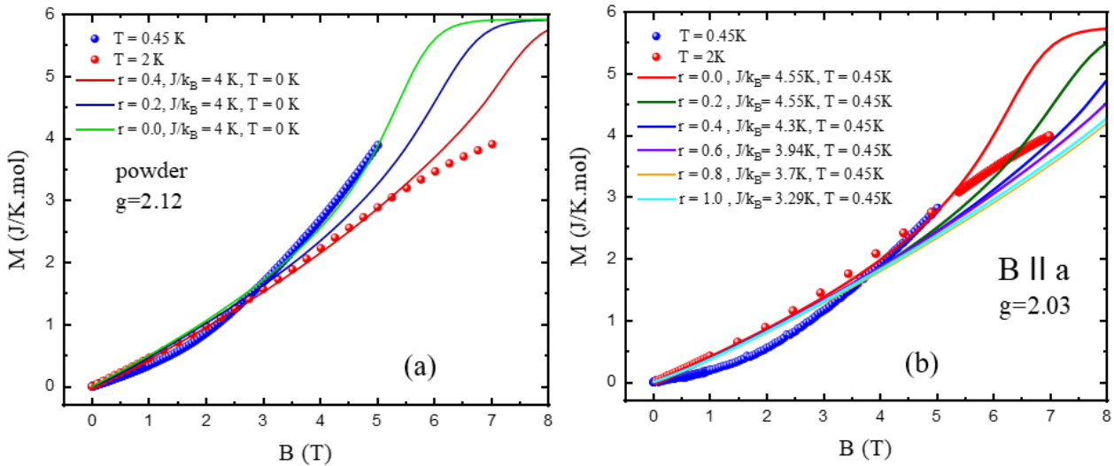
Fig. 4 Comparison between experimental isothermal magnetization of \text{Cu}(\text{tn})\text{Cl}_2 measured at fixed temperatures at 0.45 K and 2 K. Solid lines represent theoretical predictions for the S = 1/2 Heisenberg antiferromagnet on the rectangular lattice at 0.1 J/k_B [6].
