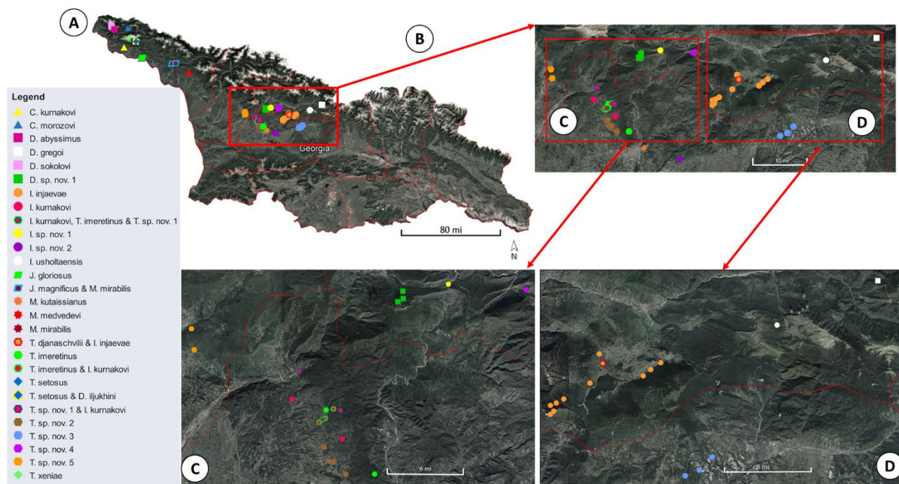
Figure 2. (A) Distribution of cave-dwelling Trechini beetles in Georgia, based on the results of the present study; (B–D) distribution in the study area.
